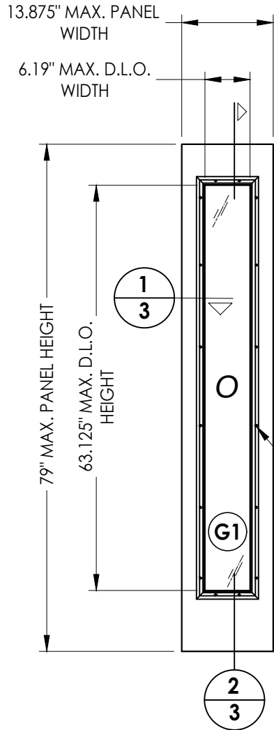
50 FIBERGLASS SIDELITE PANEL TKI PRODUCTS LITE FRAME
