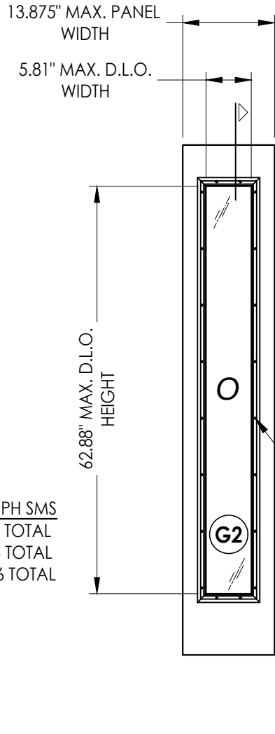
50 FIBERGLASS SIDELITE PANEL ODL LITE FRAME (EVOLVE)
